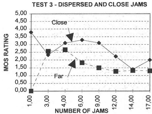
Figure 9 Test 3 for far apart and close Jams from 1 to 17 Jams with a muting error correction scheme at threshold 2.
