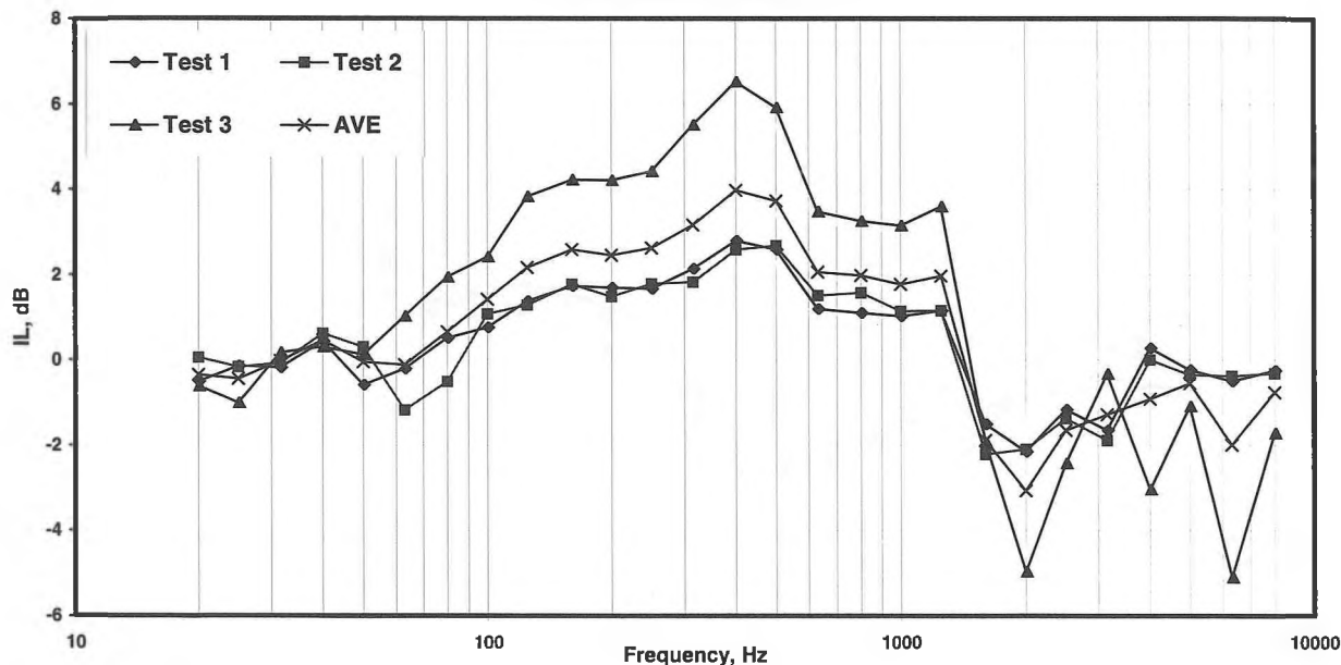
Figure 1B. Supra-aural, three tests ACTIVE IL
