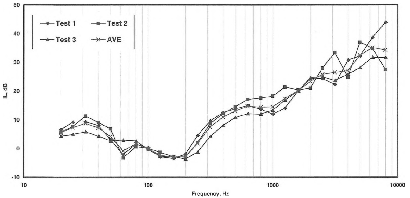
Figure 2A. Circumaural, PASSIVE IL
