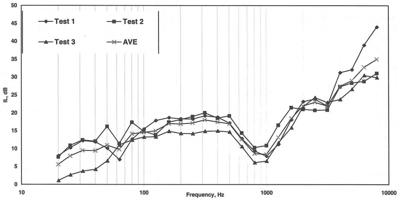
Figure 2C. Circumaural, TOTAL IL,
