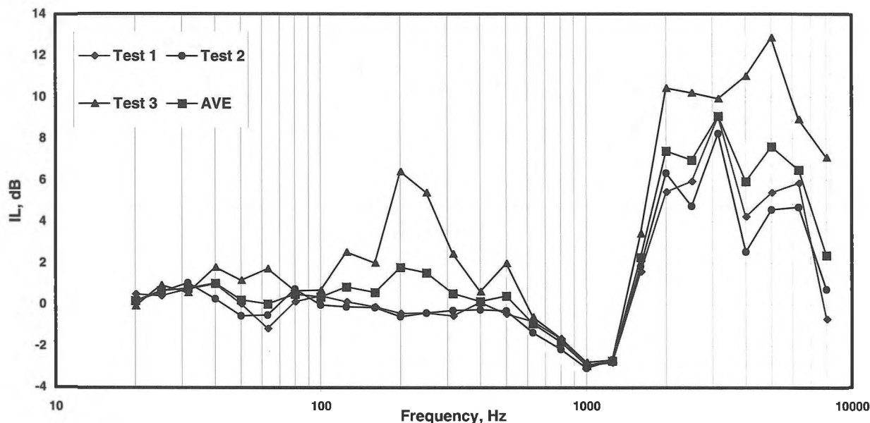
Figure 1A. Supra-aural, three tests, PASSIVE IL
