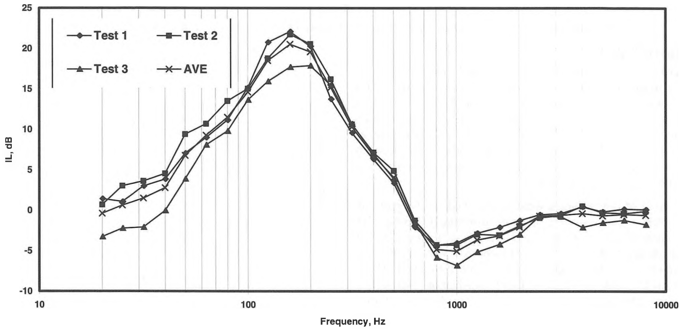
Figure 2B. Circumaural, ACTIVE IL,
