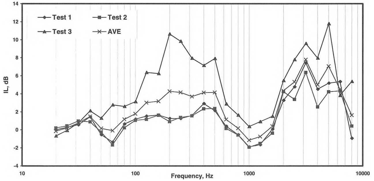
Figure 1.C Supra-aural, TOTAL IL
