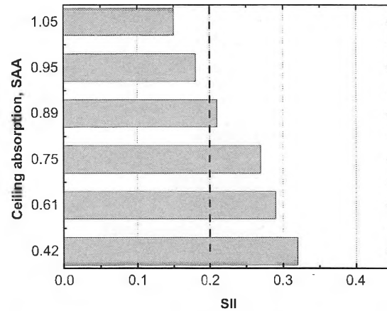
Figure 1. Effect of varied ceiling absorption on Base case.
