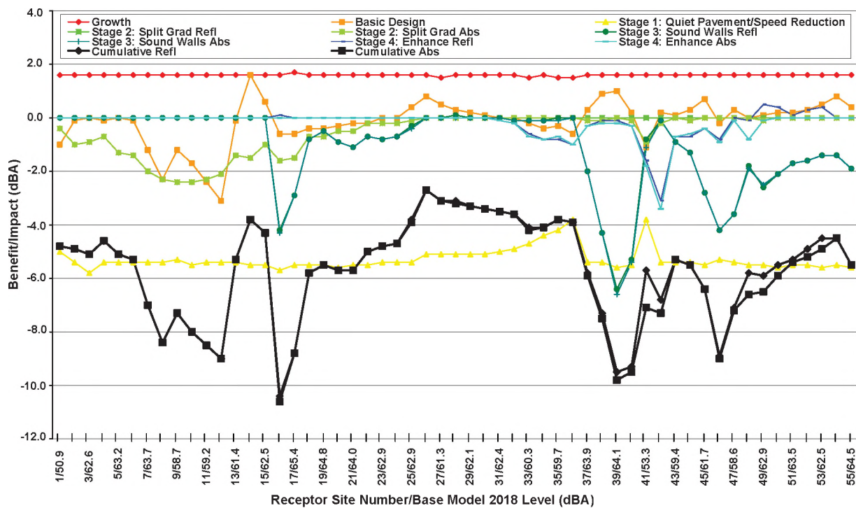
Figure 3.1: Noise Benefit/Impact vs Residential Site Number - Higher Side on Mountain Slope
