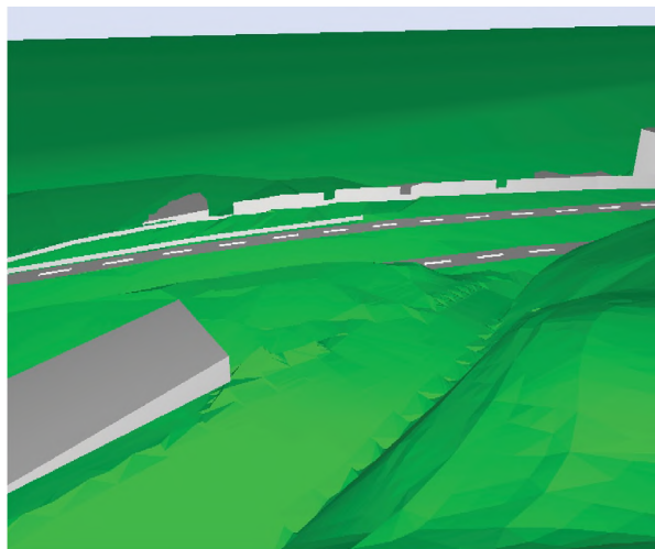
Figure 3.4a: View from Site 43 from Base Model Existing Two Lane Configuration showing Screening of Near Lane by Top-of-Cut and the Details of a Weathered Wooden Fence to be Replaced under Stage 1 Mitigation.
