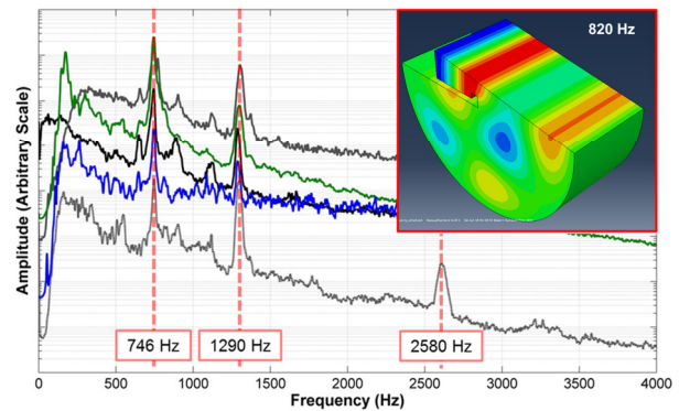
Figure 2: Measured Aeroacoustic Cavity Noise with FEA Prediction.
