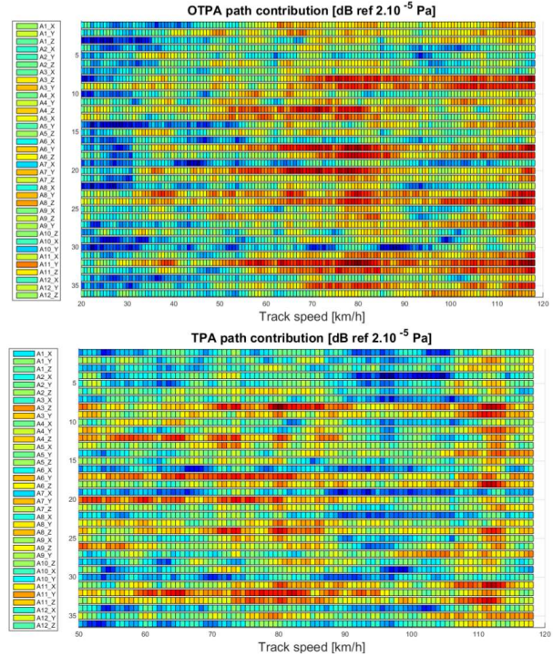
Figure 3 : Contribution of transfer paths in the case of OTPA and TPA, for the order 8 (TPA results are given from 50 km/h, whereas OTPA results start from 20 km/h).
