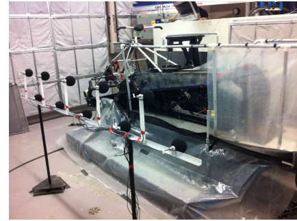
Figure 1 : Test workbench for the measurements.
