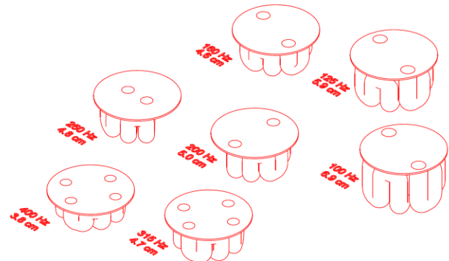
Figure 1: Drawings of the investigated sound absorbers.
