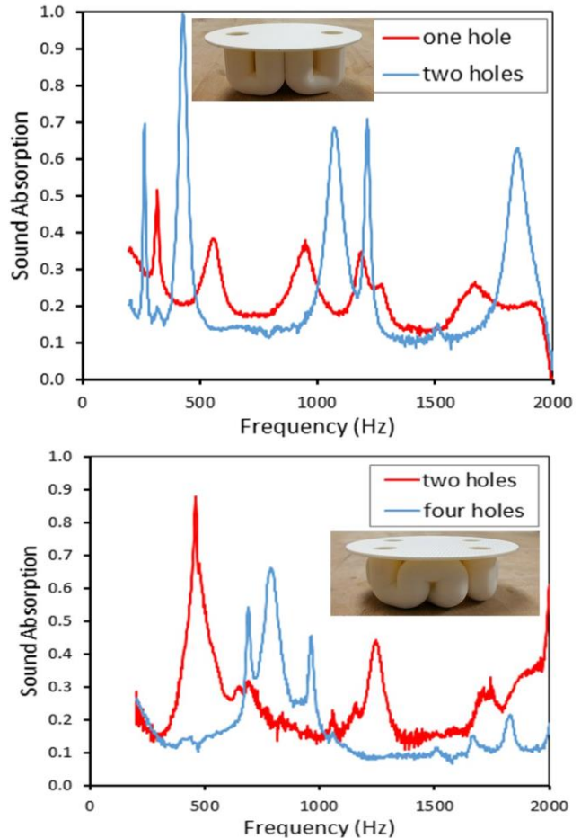
Figure 3: Sound absorption results for samples #2 and #3.
