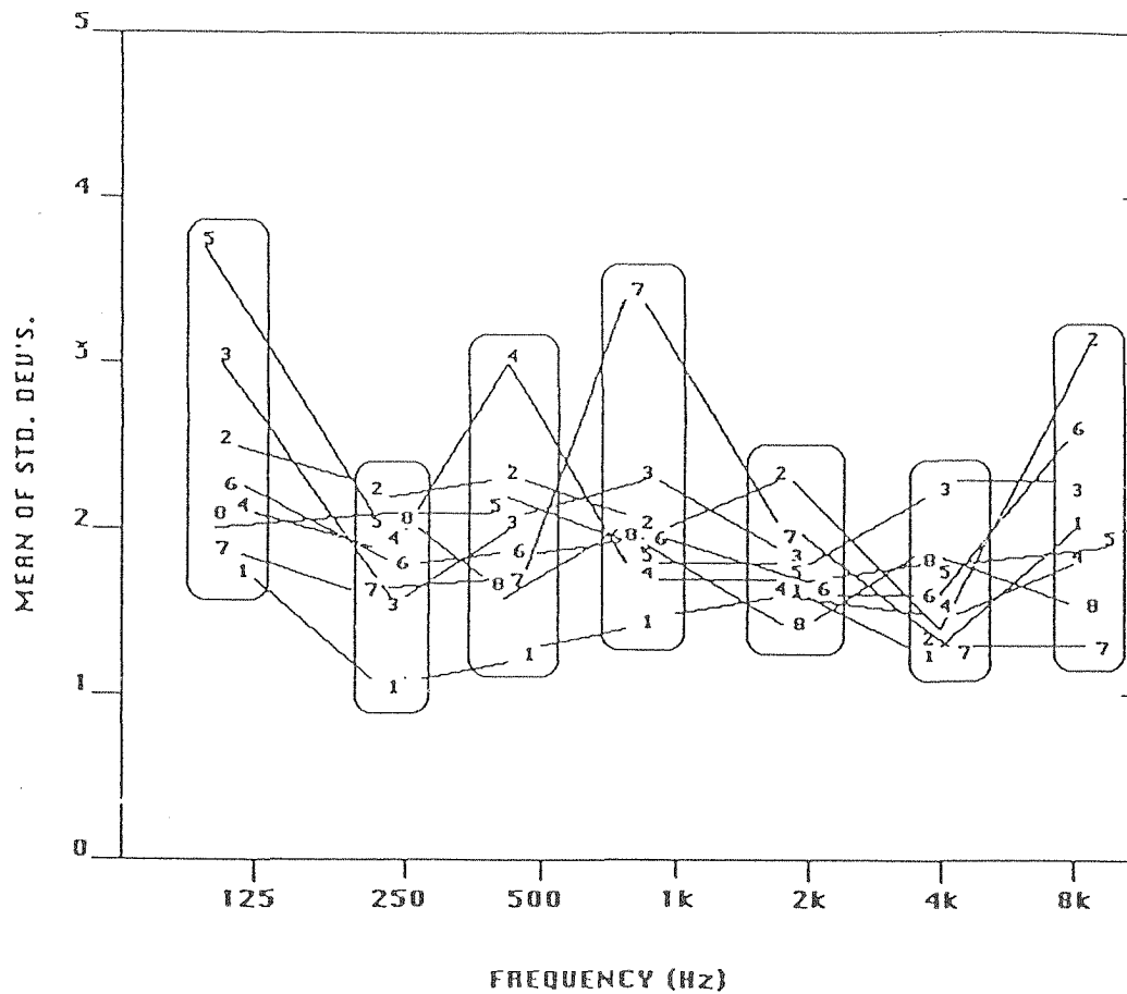
Fig. 9 Mean Standard Deviations for REAT Results for Eight Subjects Over Ten Hearing Protectors
