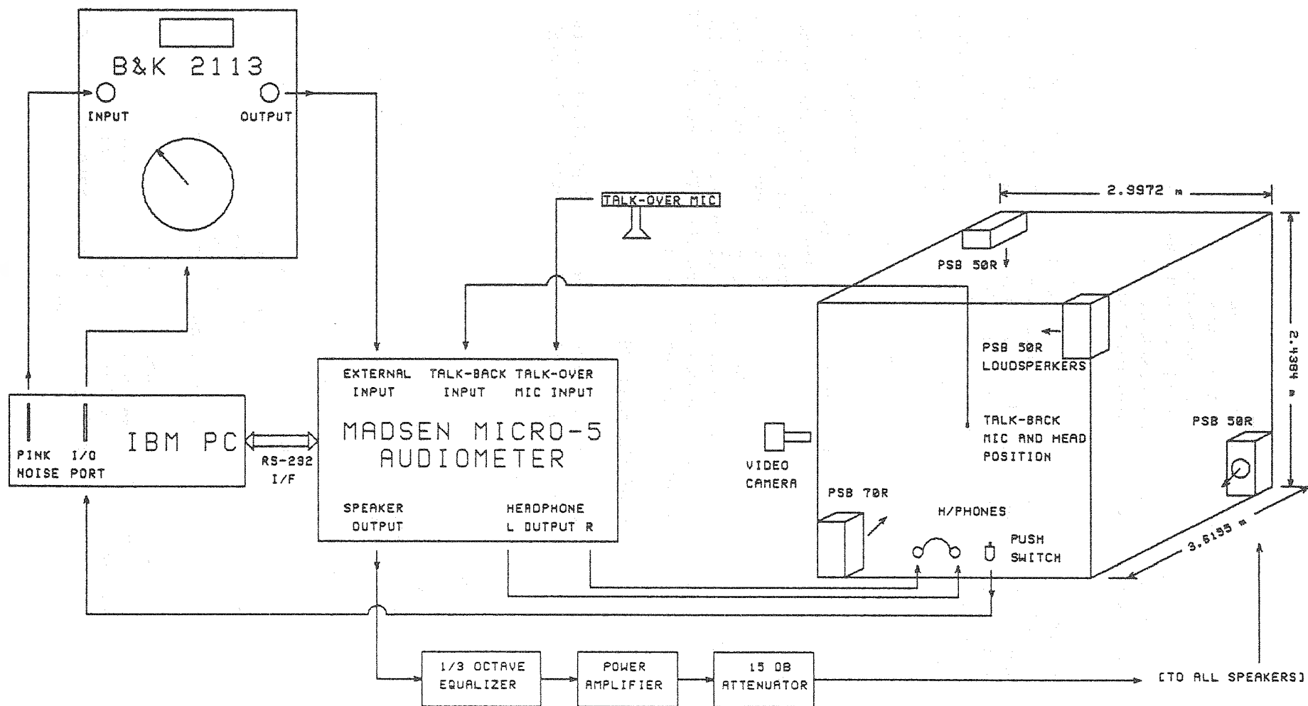
Fig. 1 Hearing Research Chamber Equipment Arrangement
