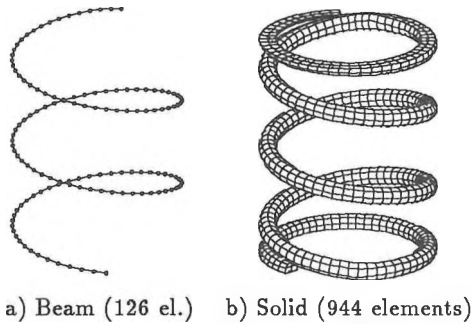
Figure 3: FE Models of helical compression spring
